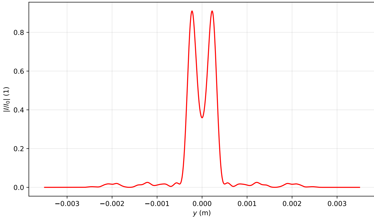
Intensity profile I(x=0, y, z=2.627)/I_0 , P_{in}=3.5P_{cr} , artificial time
